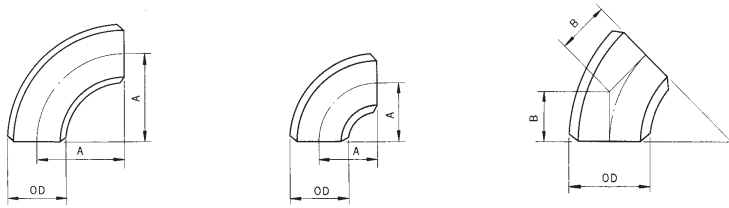
ASME B16.9
